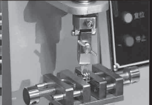
ZIPPER PULLER STRENGTH
